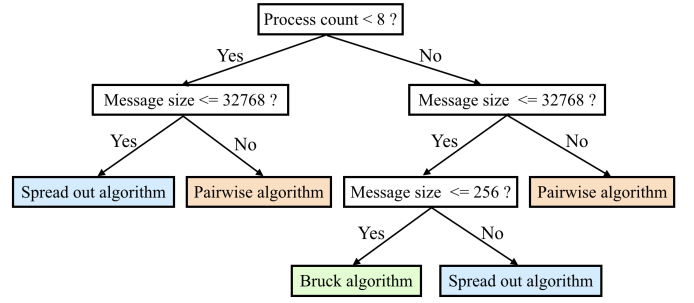
Fig. 2: The decision tree in the default configuration file of the MPICH library selects the appropriate algorithm for a given process count and message size.
